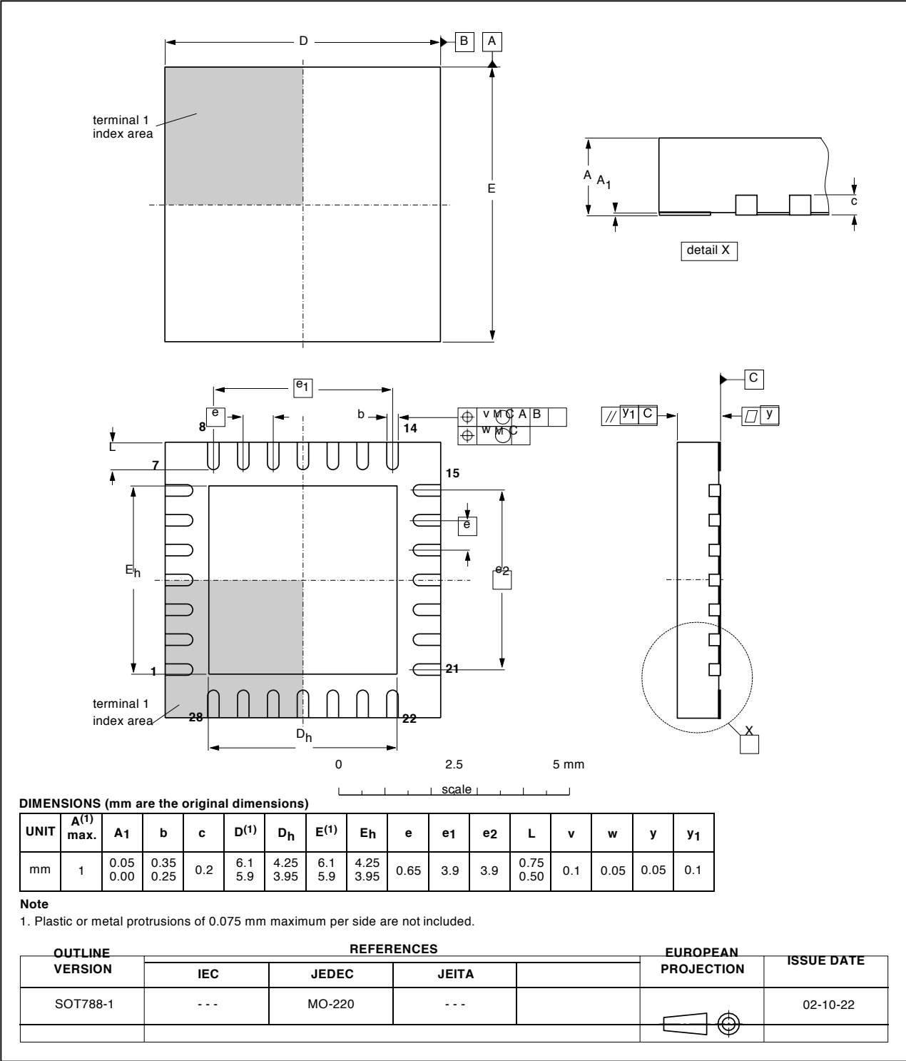
Fig 31. Package outline SOT788-1 (HVQFN28) P89LPC932A1_3 © NXP B.V. 2007. All rights reserved.
