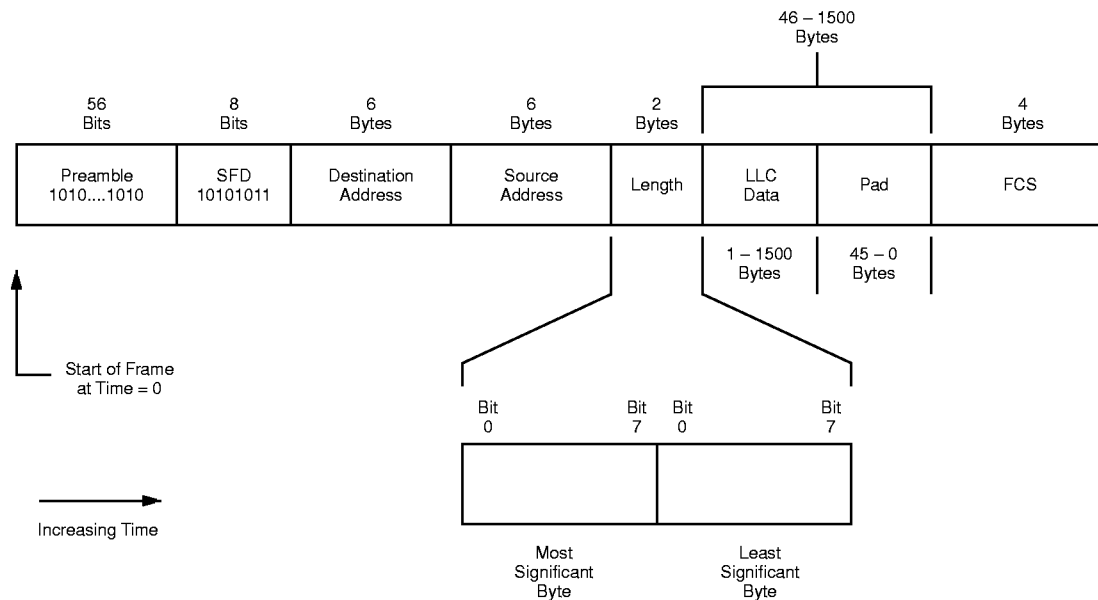
Figure 34. IEEE 802.3 Frame And Length Field Transmission Order
