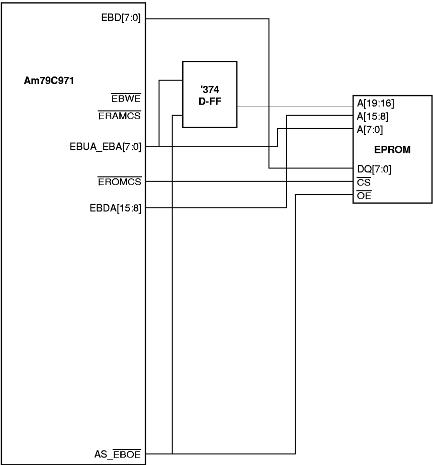
Figure 44. EPROM Only Configuration for the Expansion Bus (>64K EPROM)
