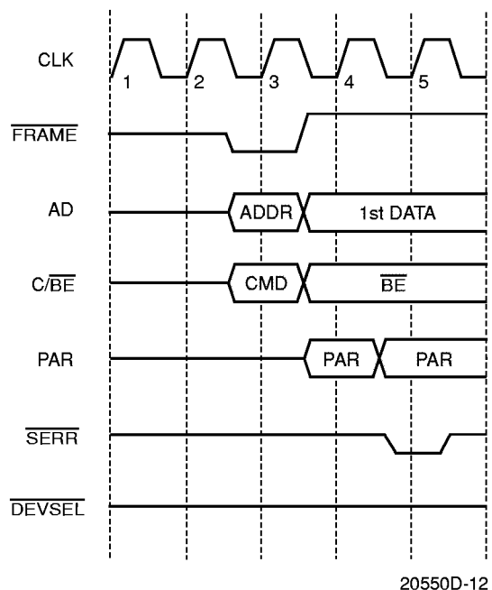
Figure 9. Address Parity Error Response
