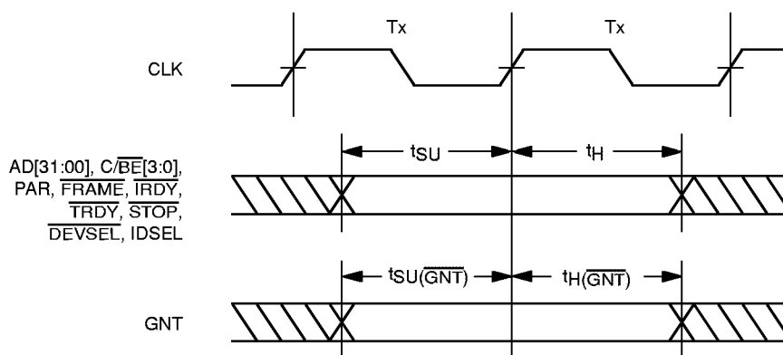
Figure 64. Input Setup and Hold Timing
