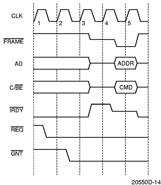
Figure 11. Bus Acquisition
