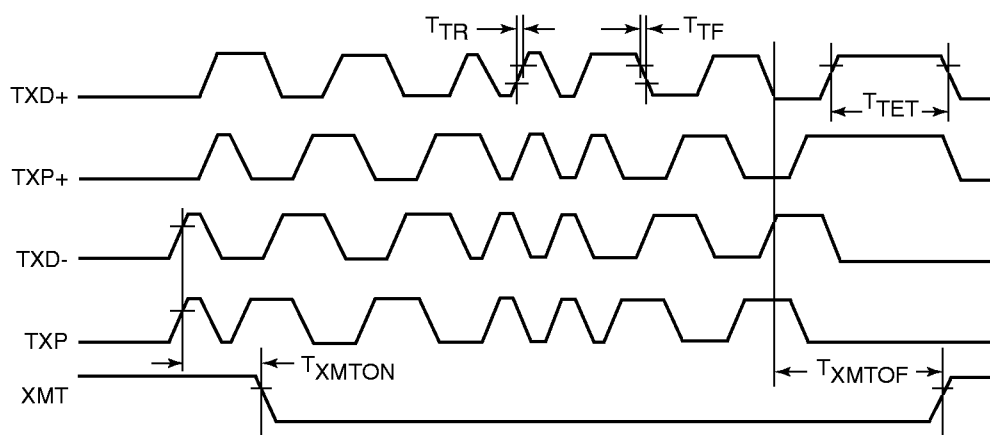
Figure 74. Transmit Timing
