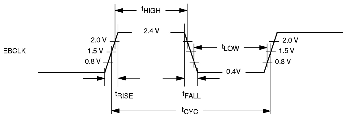
Figure 71. EBCLK Waveform
