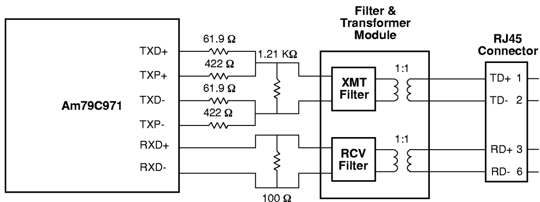
Figure 37. 10BASE-T Interface Connection
