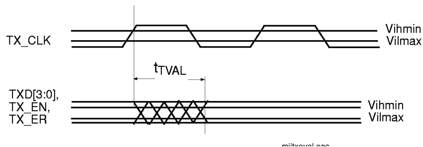
Figure 84. Transmit Timing
