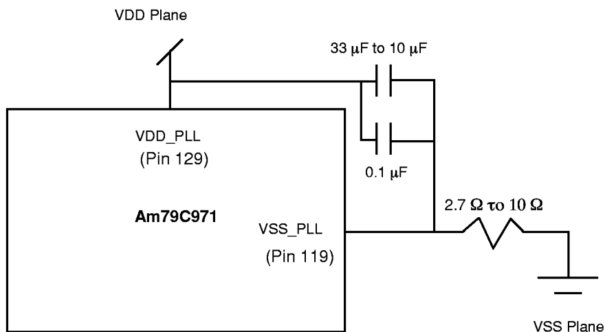
Figure B2. Power and Ground Pin Connections
