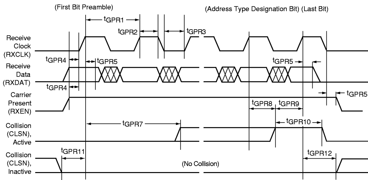
Figure 90. Receive Timing
