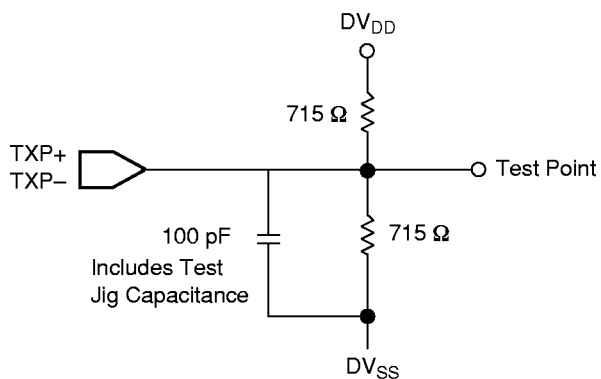
Figure 61. TXP Outputs Test Circuit
