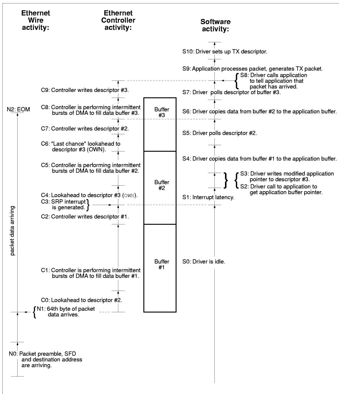
Figure D3. LAPP Timeline for Two-Interrupt Method
