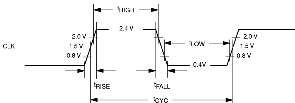
Figure 62. CLK Waveform for 5 V Signaling
