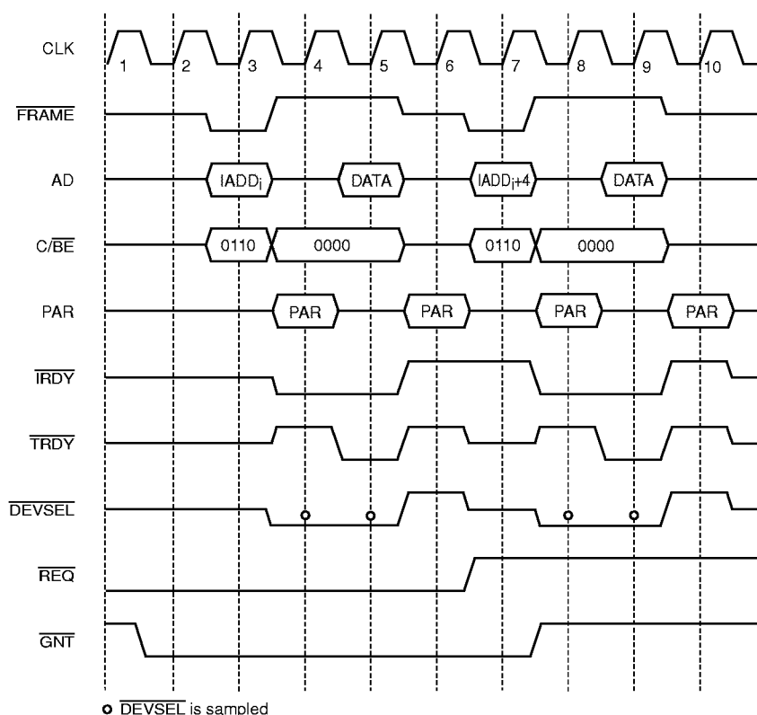
Figure 23. Initialization Block Read In Non-Burst Mode
