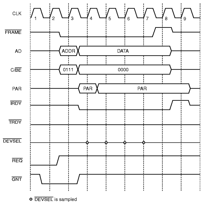
Figure 21. Master Abort
