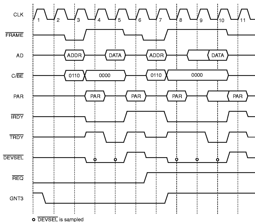
Figure 12. Non-Burst Read Transfer
