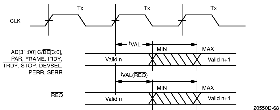
Figure 65. Output Valid Delay Timing
