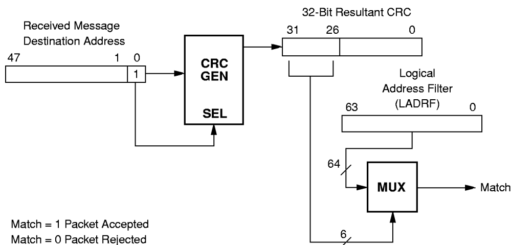
Figure 57. Address Match Logic
