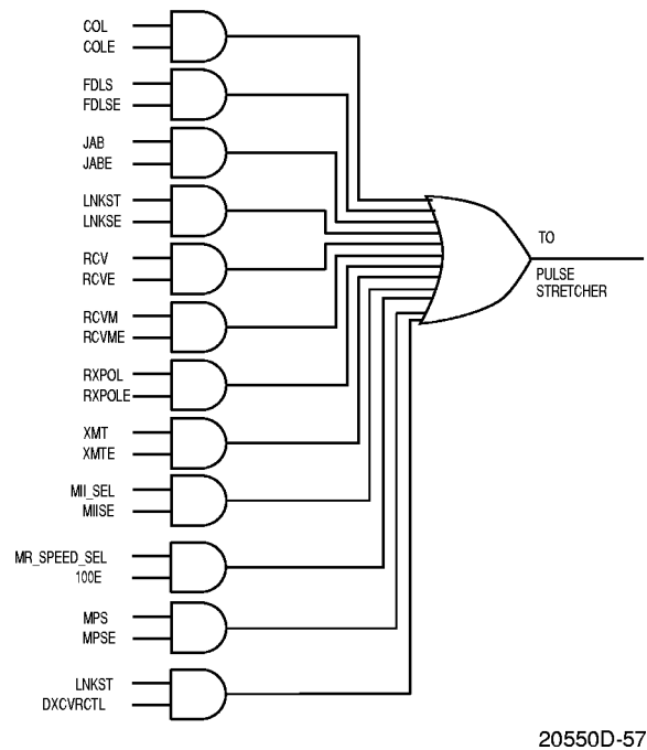
Figure 54. LED Control Logic
