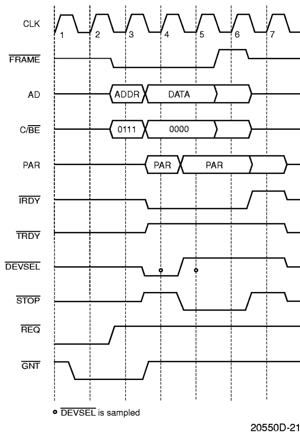
Figure 18. Target Abort
