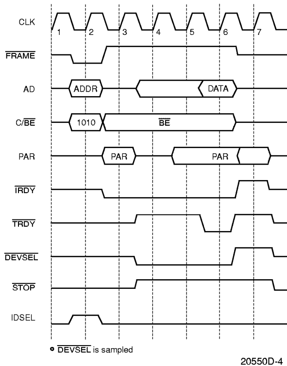
Figure 1. Slave Configuration Read
