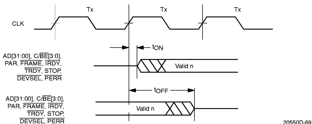
Figure 66. Output Tri-state Delay Timing
