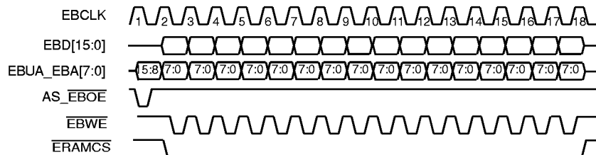
Figure 53. Typical SRAM Write Operation
