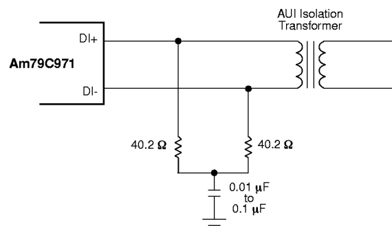
Figure 36. AUI Differential Input Termination
