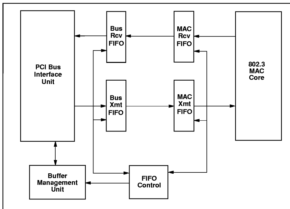
Figure 50. Block Diagram No SRAM Configuration
