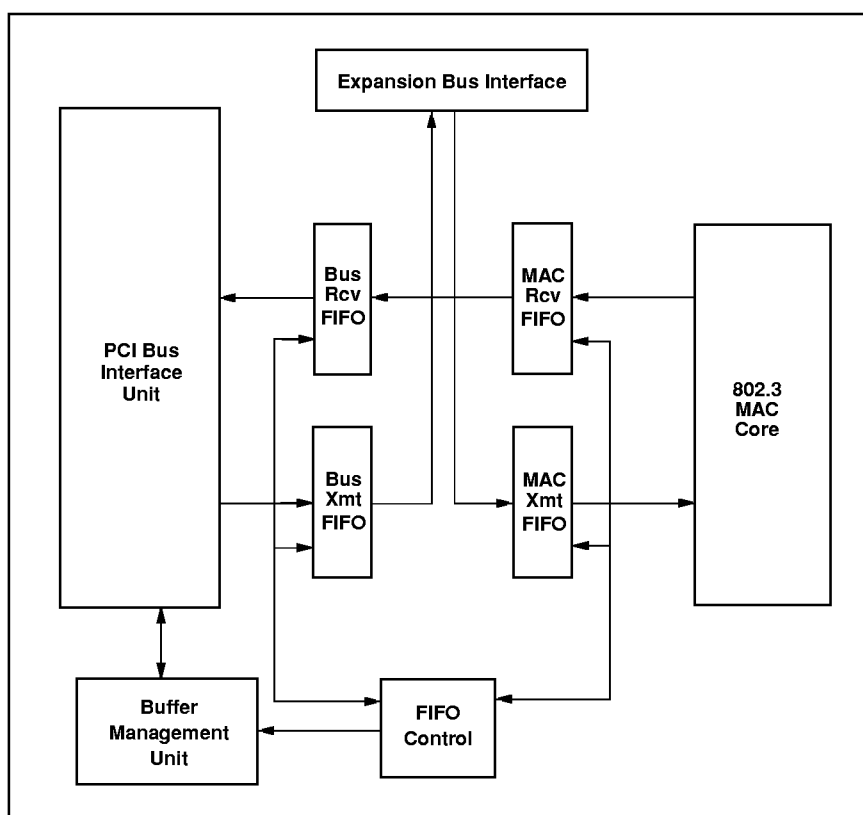
Figure 51. Block Diagram Low Latency Receive Configuration
