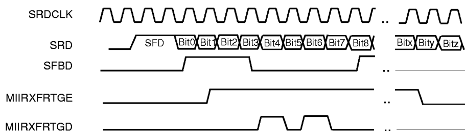
Figure 41. Internal PHY Receive Frame Tagging
