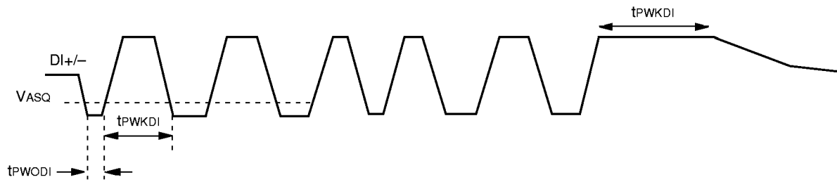
Figure 81. Receive Timing
