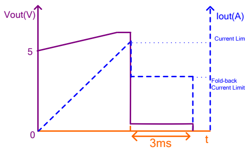
Figure 4: Over-Current Limit
