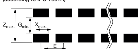
Suggested land pattern (according to IPC-7351A)
