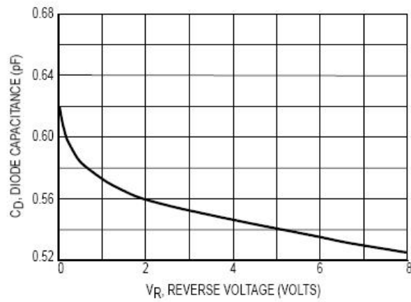
Figure 3. Capacitance
