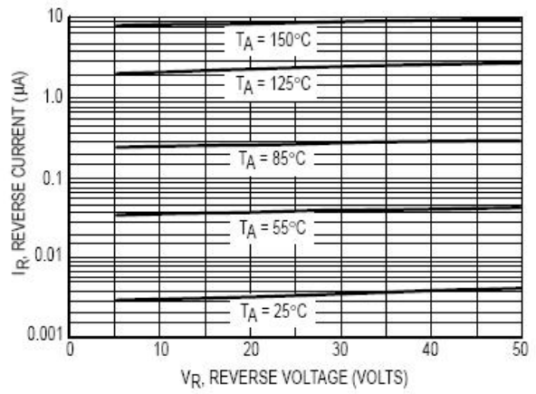
Figure 2. Leakage Current
