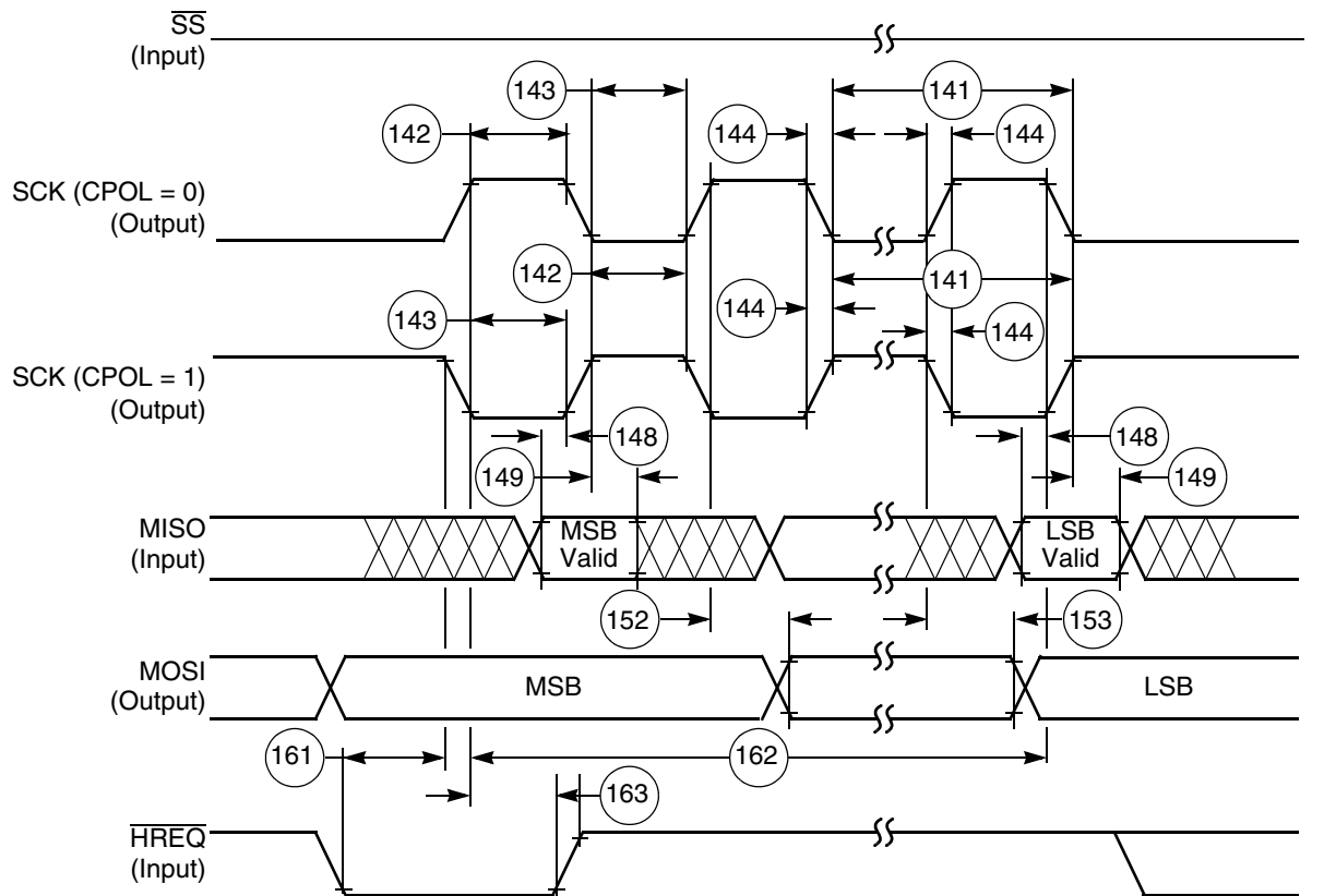
Figure 3-28 SPI Master Timing (CPHA = 1)
