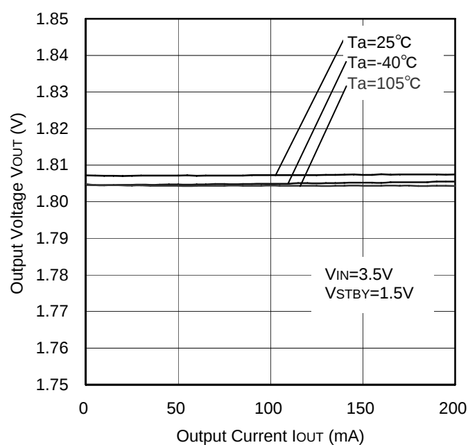
Figure 28. Load Regulation
