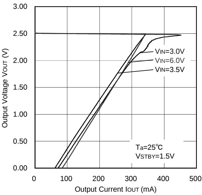
Figure 52. OCP Threshold
