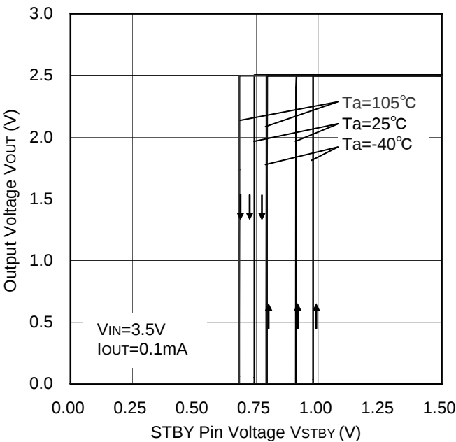
Figure 55. STBY Threshold
