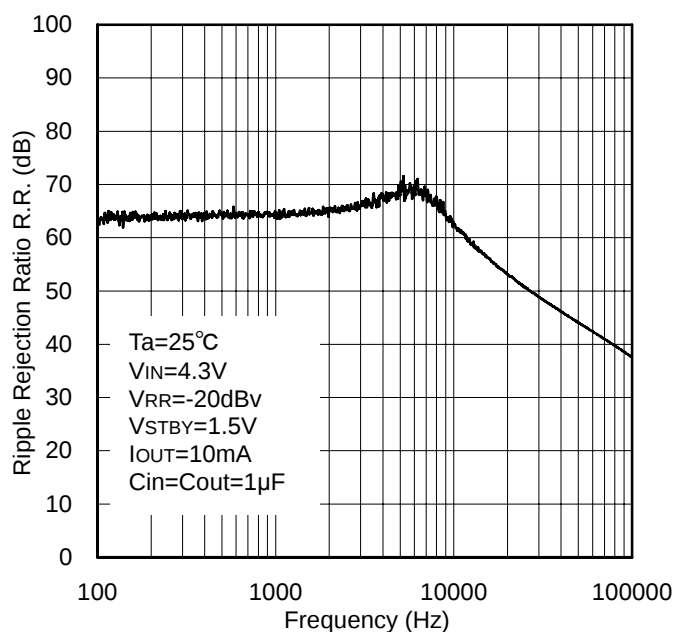
Figure 82. Ripple Rejection Ratio vs. Frequency
