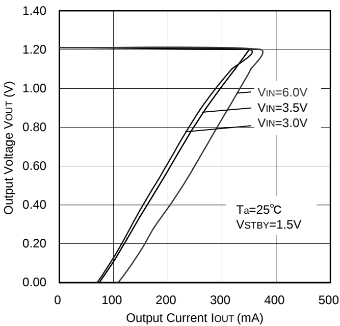
Figure 8. OCP Threshold
