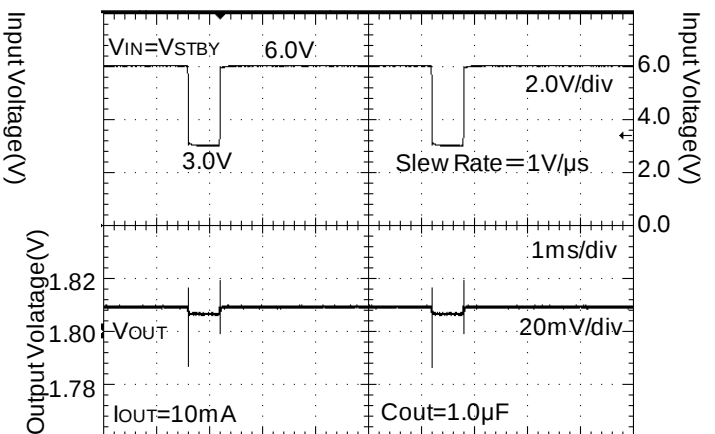
Figure 42. Line Transient Response (3.0 to 6.0V)
