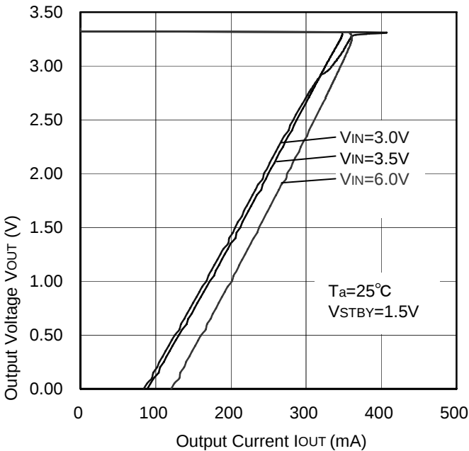
Figure 75. OCP Threshold
