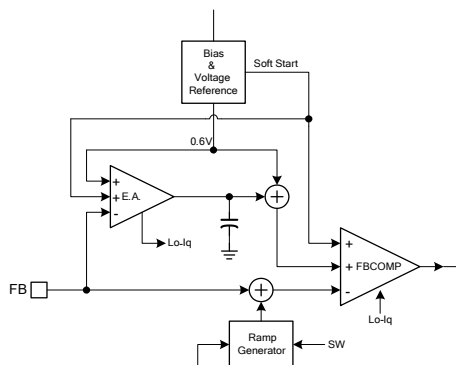
Figure 2: Operation Blocks in Sleep Mode
