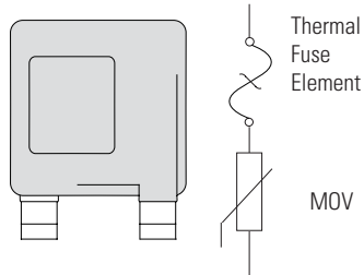
TMOV®34S Varistor "E" 2-Lead Varistor
