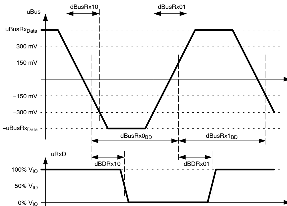
Figure 12. Reception Parameters
