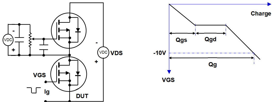
Fig.15-Gate Charge Test Circuit & Waveform
