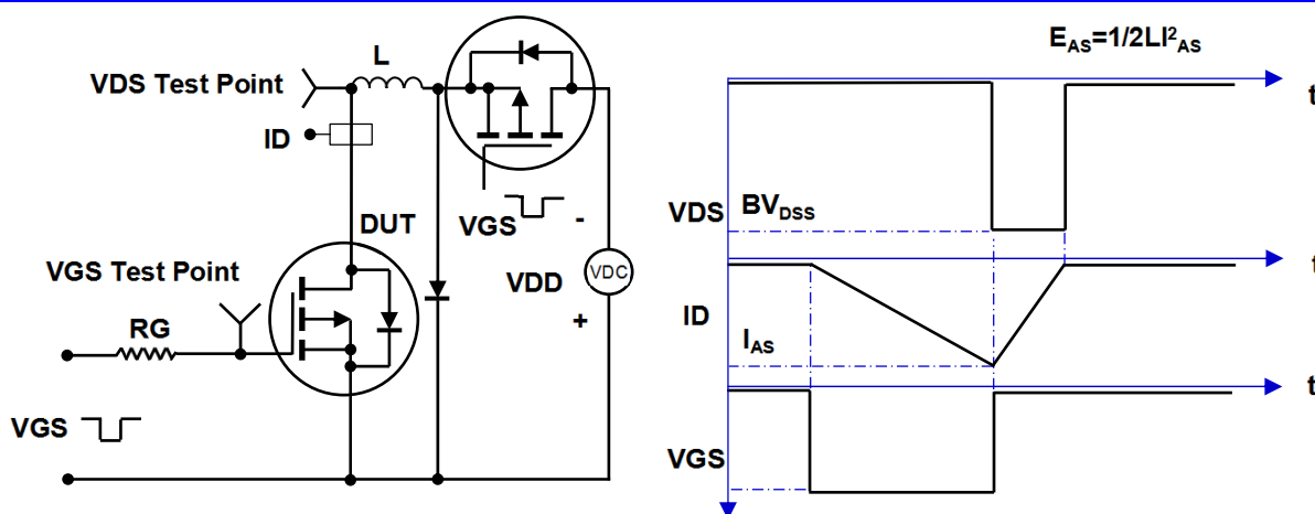
Fig.16- EAS Test Circuit & Waveform
