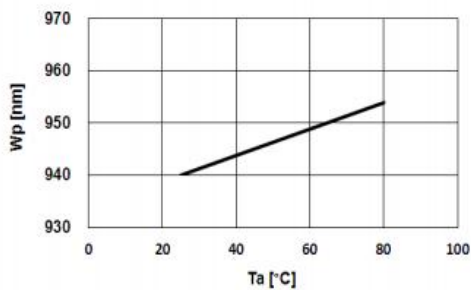
Fig.5 – Peak Wavelength (@50mA) vs. Ambient Temperature
