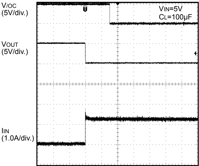
TIME(4ms/div.) Figure 37. Over-Current Response 1 \Omega Load Connected at Enable
