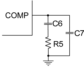
Figure 10: Compensation Network
