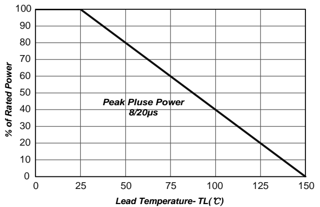
Fig2. Power Derating
