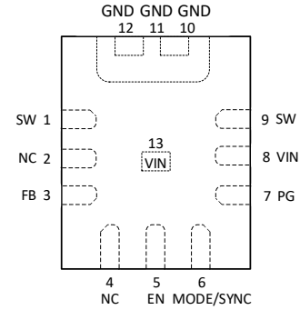
13 引脚 LQFN (2mm x 3mm)
