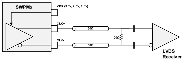
AC-Coupled LVDS
