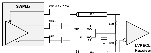
AC-Coupled Self-Biased LVEPCL - 50 Ω w/VTT Bias
