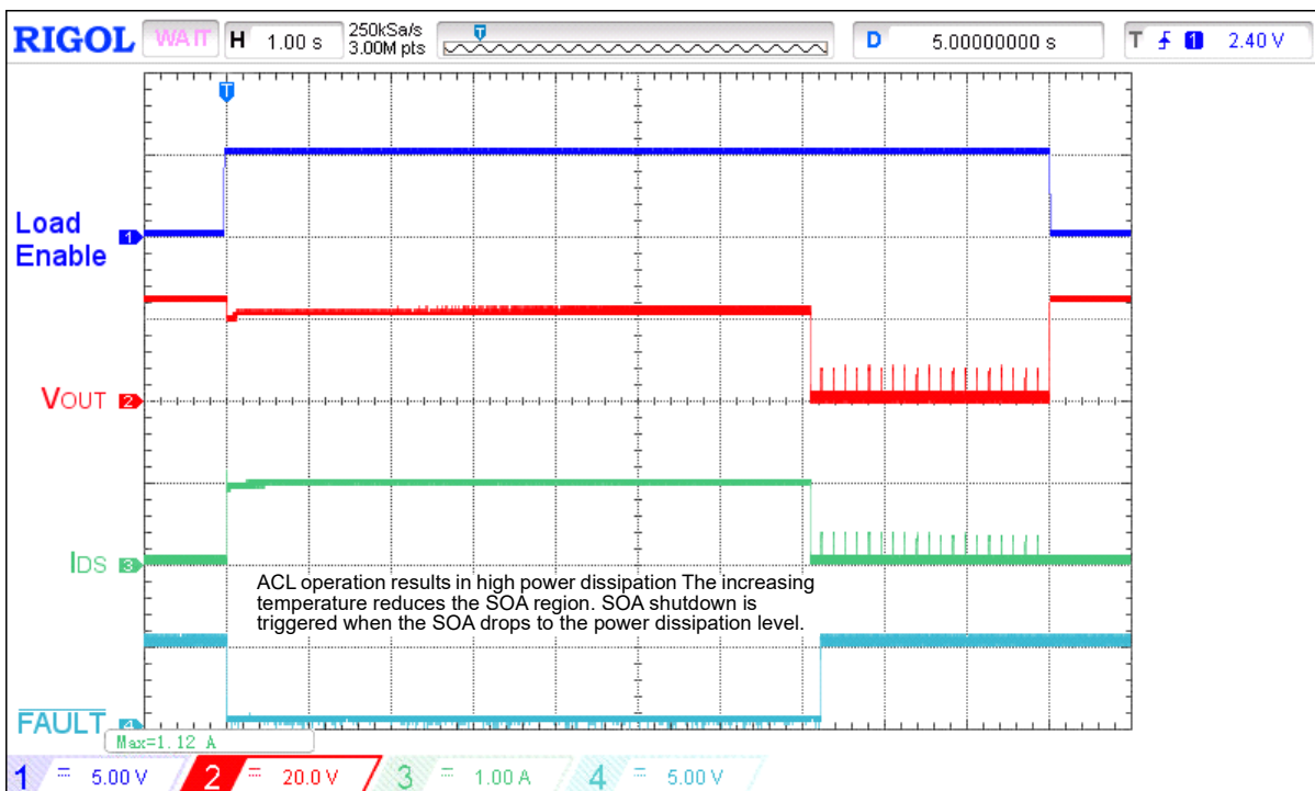
Figure 12. Thermally induced SOA shutdown for V_{IN} = 24\text{ V} , C_{LOAD} = 10\ \mu\text{F} , R_{SET} = 91\text{ k}\Omega , I_{ACL} = 1\text{ A} , R_{LOAD} = 20\ \Omega ,
