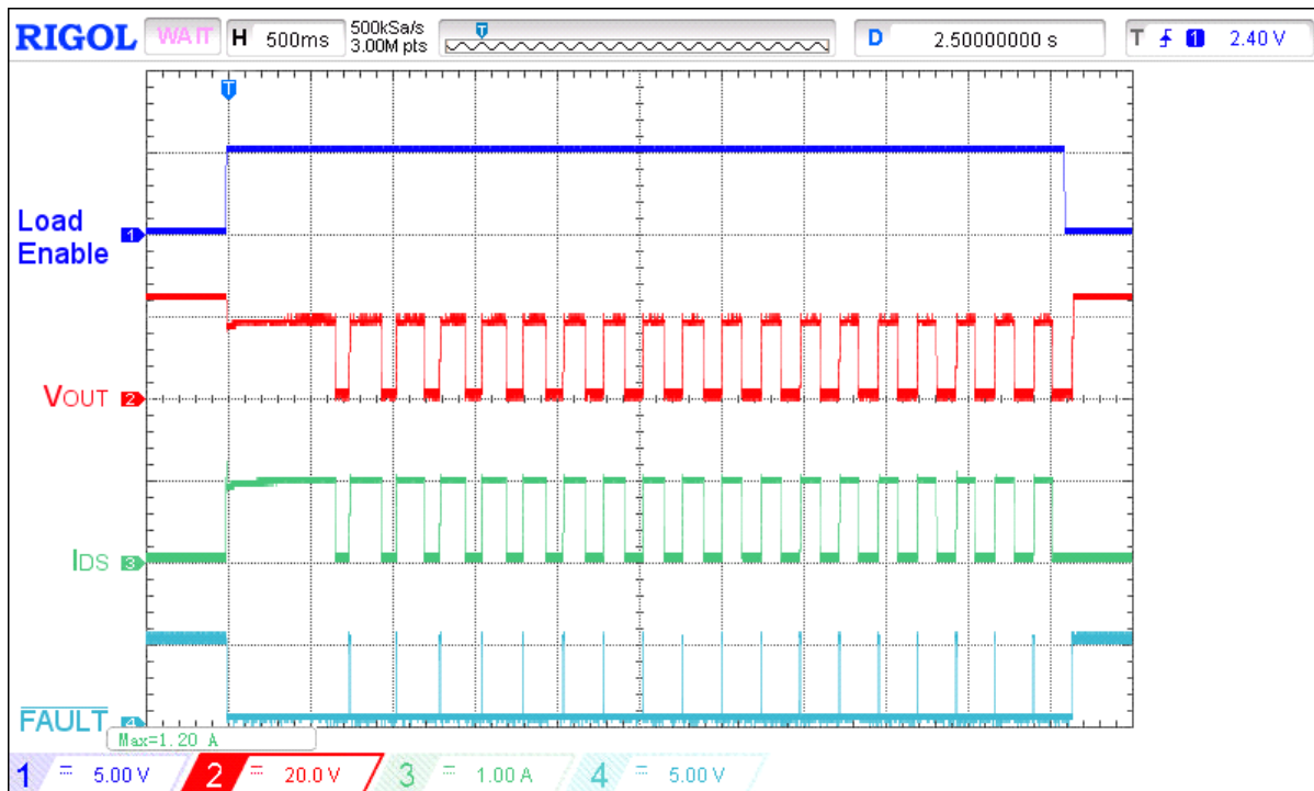
Figure 11. Typical ACL operation waveform for V_{IN} = 24\text{ V} , C_{LOAD} = 10\ \mu\text{F} , I_{ACL} = 1\text{ A} , R_{SET} = 91\text{ k}\Omega
