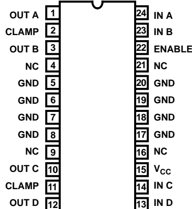
CA3262A (SOIC) TOP VIEW PRELIMINARY
