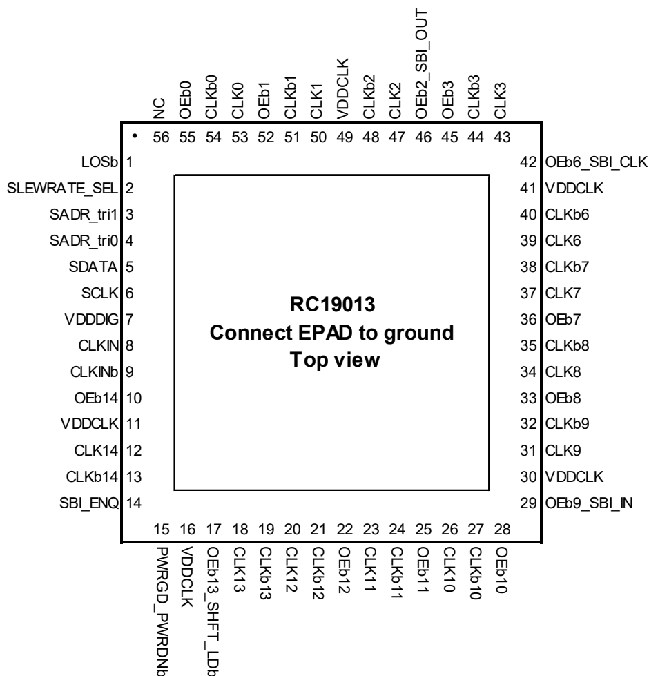
Figure 6. RC19013 56-VFQFP – Top View
