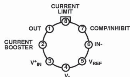
CA3085S, AS, BS (CAN) TOP VIEW
