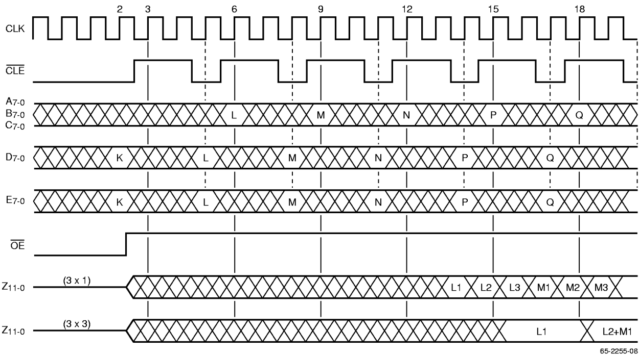
Figure 5. 3xX Modes, Periodic Long \overline{CLE} Pulses
