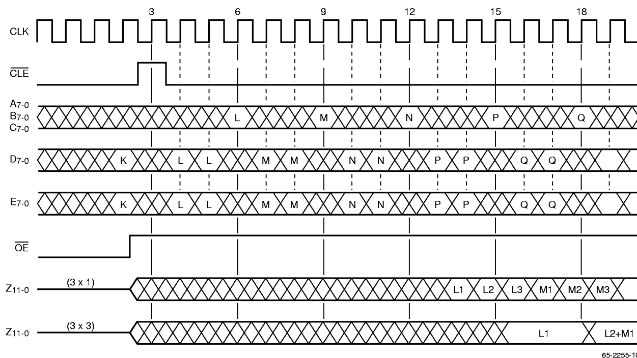
Figure 7. 3xX Modes, Single \overline{\text{CLE}} Rising Edge
