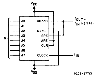
Fig. 18 - Divide-by-"N" counter.
