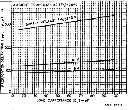
Fig. 6 — Typical propagation delay time as a function of load capacitance (clock to CO/ZD).
