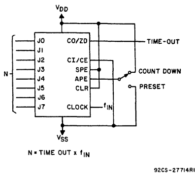
Fig. 19 - Programmable timer.
