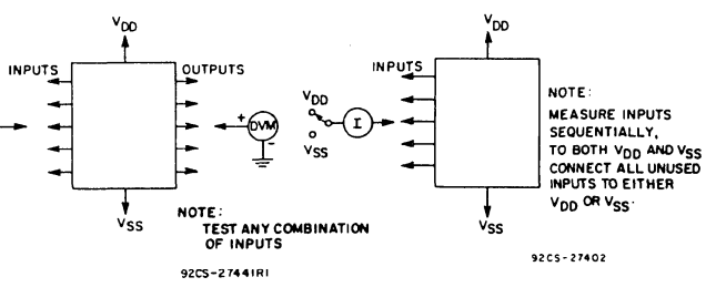
Fig. 10 — Input voltage test circuit. Fig. 11 — Input current test circuit.
