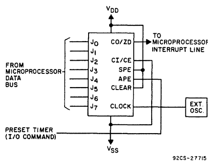
Fig. 20 - Microprocessor interrupt timer.
