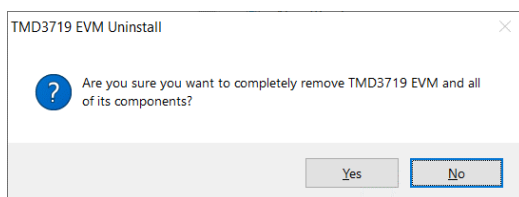
Figure 9: Remove Installation
