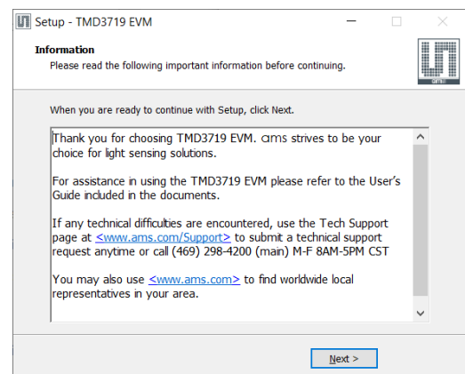
Figure 7: Information Screen
