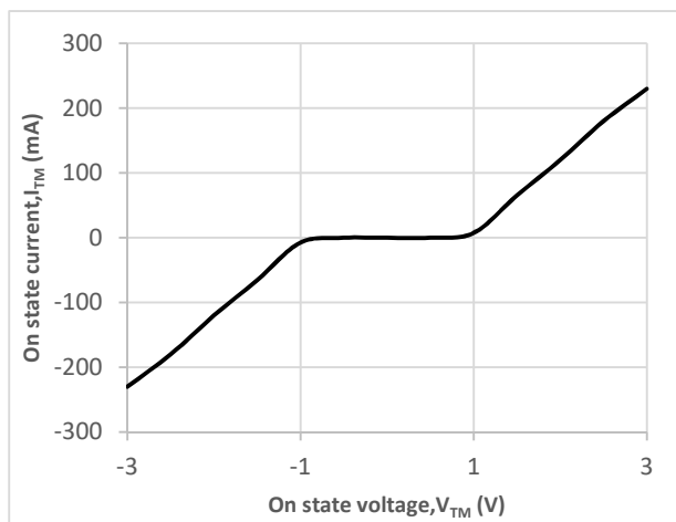
Fig.2 On-state characteristic
