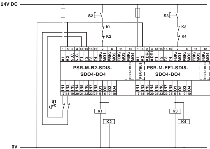
Application drawing
