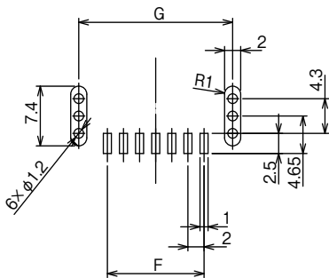
Recommended PCB Dimensions (Connector Side)
