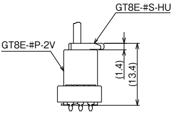
Diagram of Mating Condition During Use
