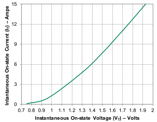
Figure 4: On-State Current vs. On-State Voltage (Typical)
