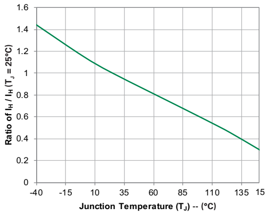
Figure 3: Normalized DC Holding Current vs. Junction Temperature
