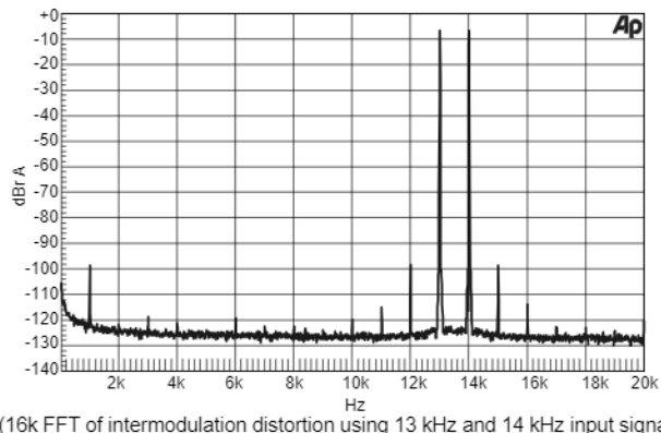
Figure 34. Twin Tone IMD FFT (HRM)
