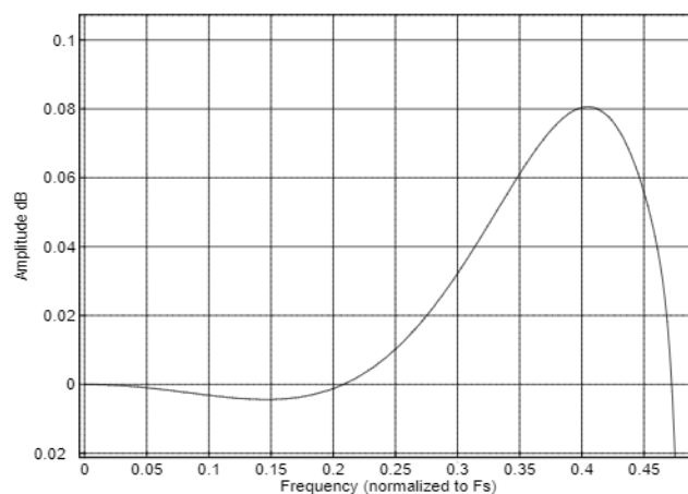
Figure 20. Passband Ripple
