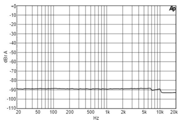
Figure 30. THD+N vs. Frequency (BRM)
