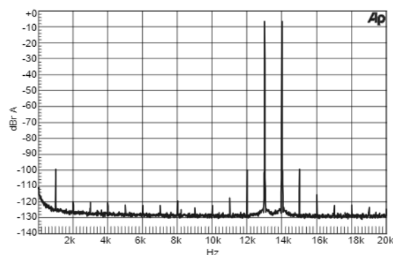
Figure 28. Twin Tone IMD FFT (BRM)
