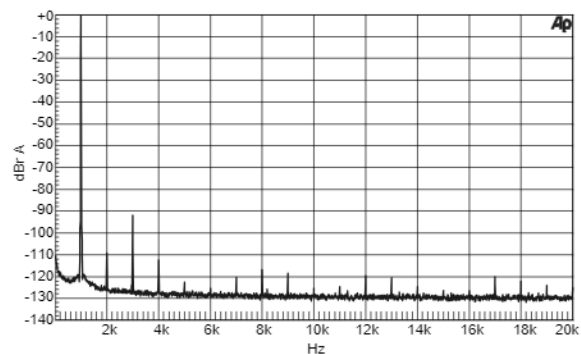
Figure 25. 0 dBFS FFT (BRM)
