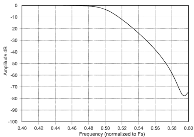
Figure 22. Transition Band
