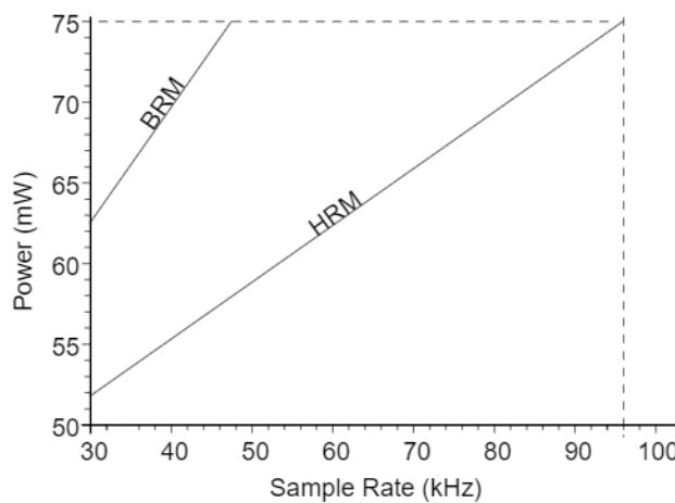
Figure 3. Power vs. Sample Rate
