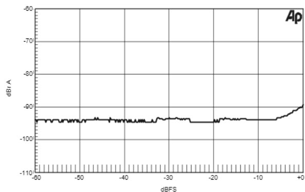
Figure 29. THD+N vs. Amplitude (BRM)
