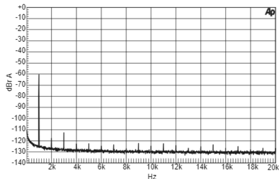
Figure 26. -60 dBFS FFT (BRM)
