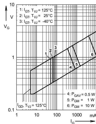
Fig. 5 Gate trigger range
