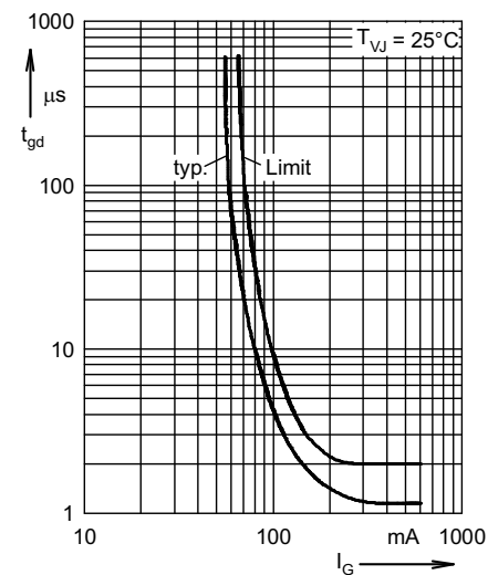
Fig. 7 Gate controlled delay time
