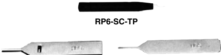
RP6-SC-TP RP13-PC-TP RP13A-SC-TP Extraction tools
