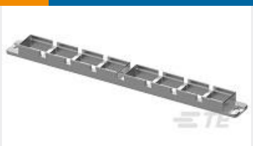
TE Part #2226784-4 FORTIS LRM, BACKPLANE, 8 BAY SHELL
