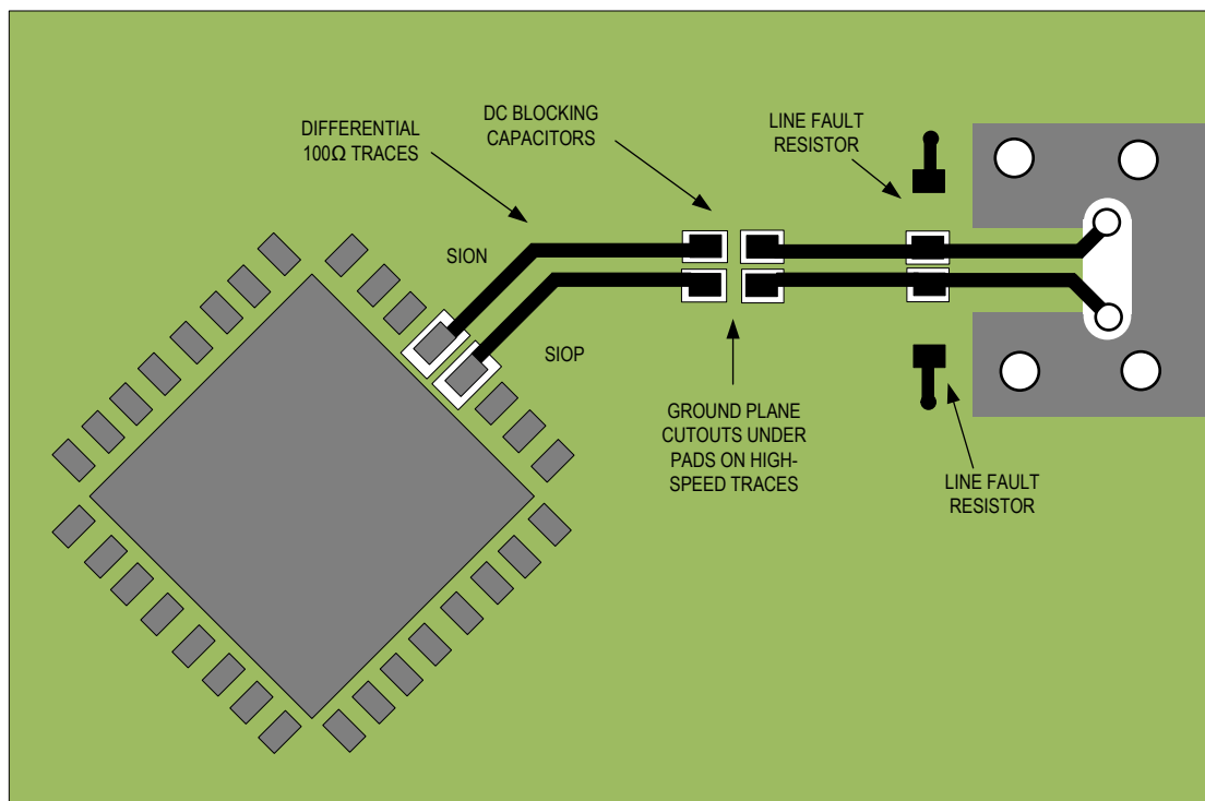
Figure 31. STP Layout Example
