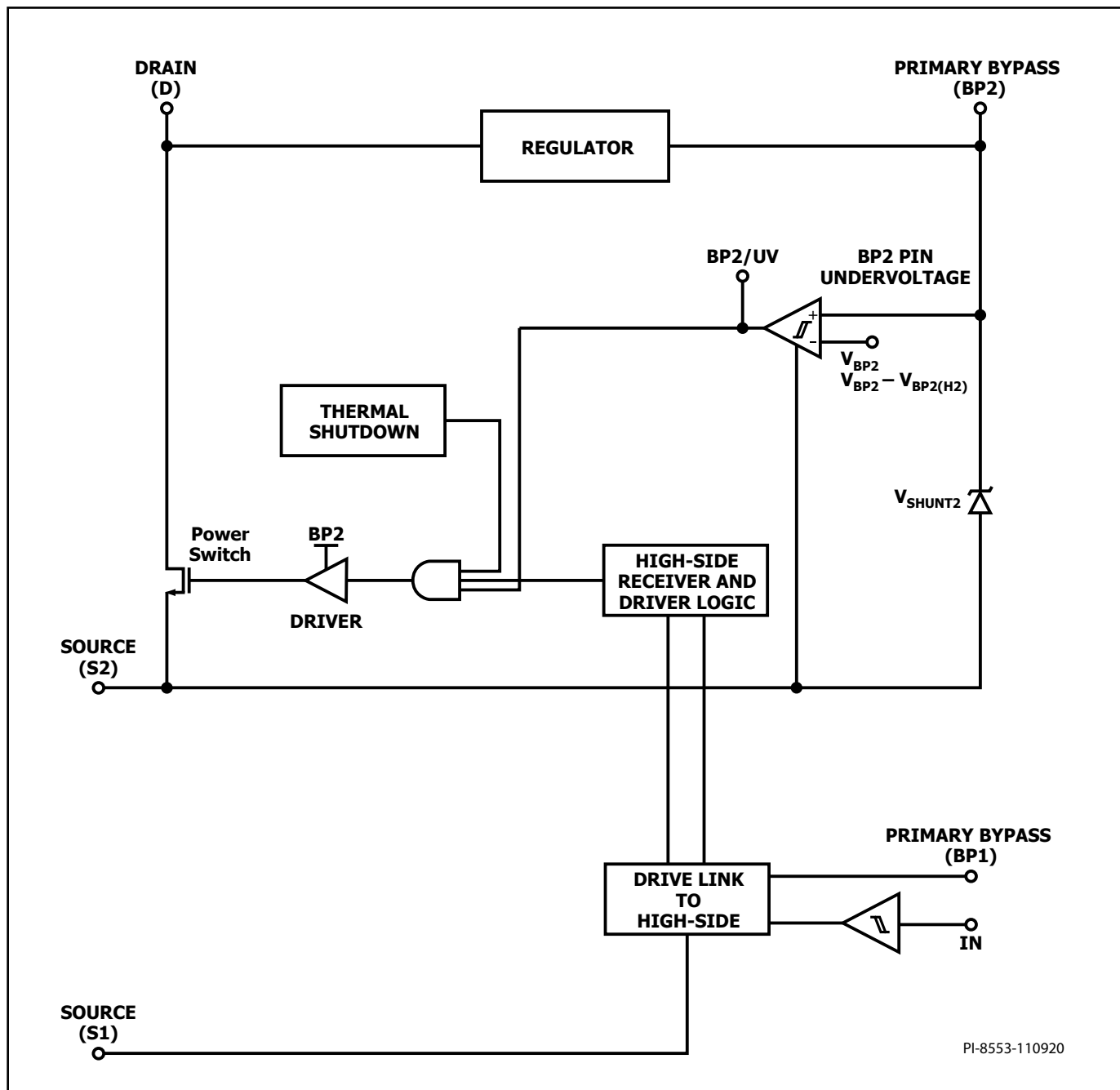
Figure 3. Block Diagram.
