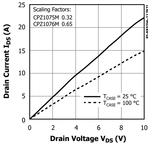
Figure 14. Optional Characteristics.
