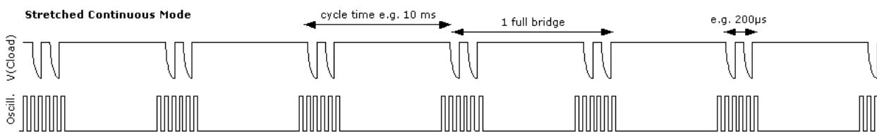
Figure 3-18: Stretched continuous mode
