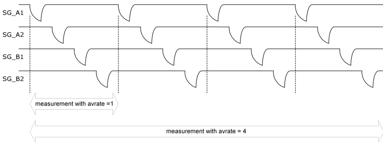
Figure 3-15: Averaging
