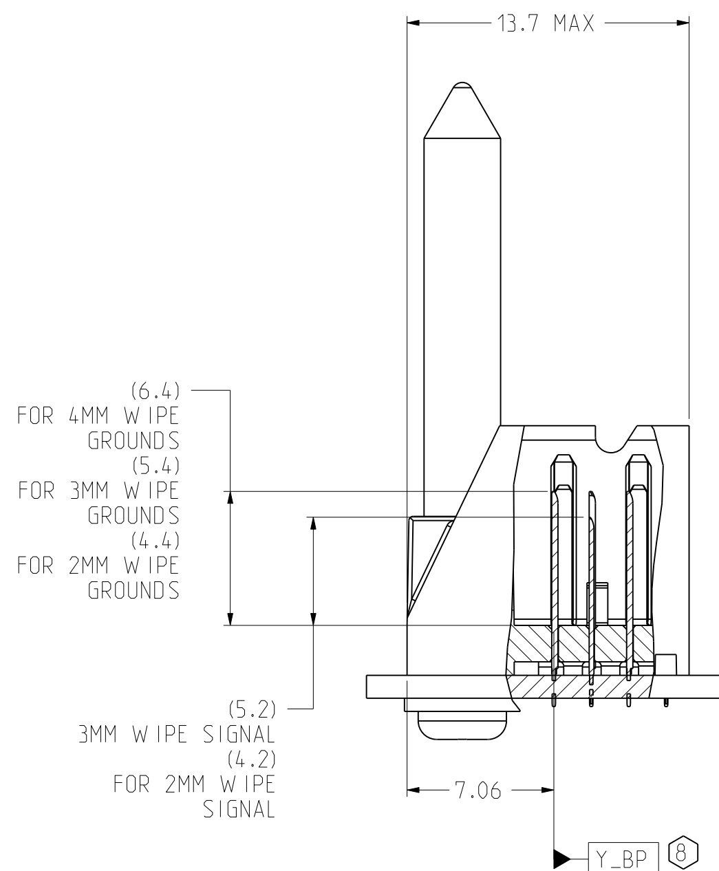
SECTION Z-2
