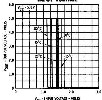
Fig. 22 OUTPUT VOLTAGE VERSUS ASYNCHRONOUS INPUT VOLTAGE
