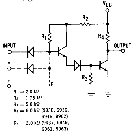
Fig. 2—BASIC GATE CIRCUIT
