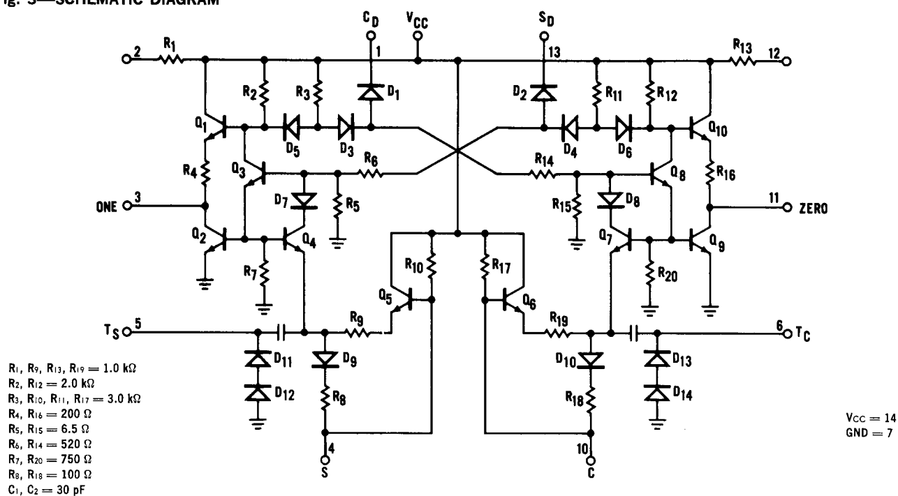
Fig. 3—SCHEMATIC DIAGRAM
