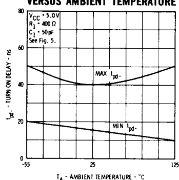
Fig. 4h WORST CASE TURN ON DELAY VERSUS AMBIENT TEMPERATURE
