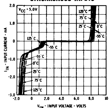
Fig. 18 INPUT CURRENT VERSUS INPUT VOLTAGE SYNCHRONOUS INPUTS
