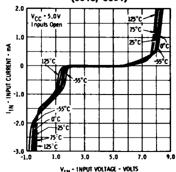
Fig. 14 INPUT CURRENT VERSUS INPUT VOLTAGE - CLOCK INPUT (9948, 9094)
