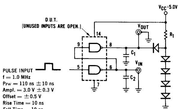
Fig. 7— t_{pd} TEST CIRCUIT AND WAVEFORMS
