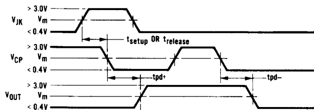
Fig. 31—WAVEFORMS
