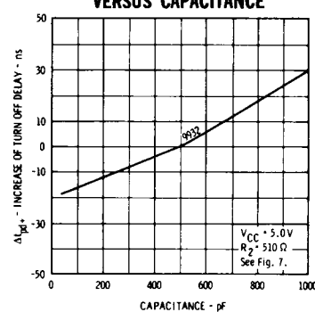
Fig. 10c INCREASE OF TURN OFF DELAY VERSUS CAPACITANCE
