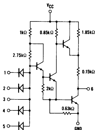
Fig. 2—SCHEMATIC DIAGRAM OF THE DT μ L 9932 ELEMENT (ONE GATE)
