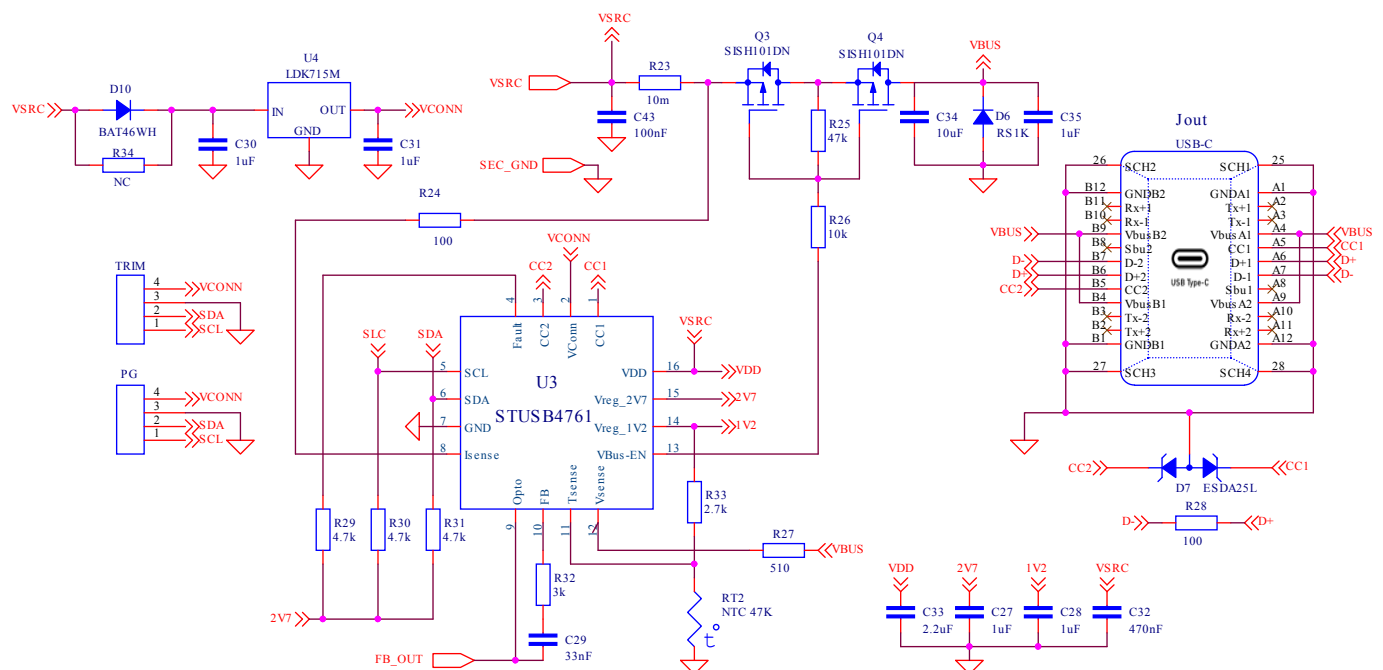
Figure 4. Daughterboard schematic
