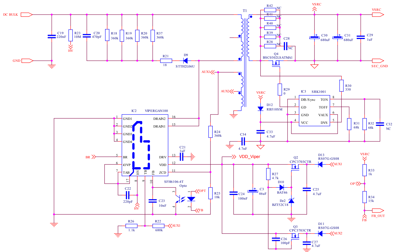
Figure 3. Flyback stage schematic
