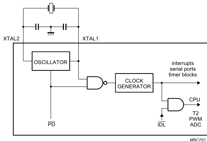
Fig.13 Internal Idle and Power-down clock configuration.
