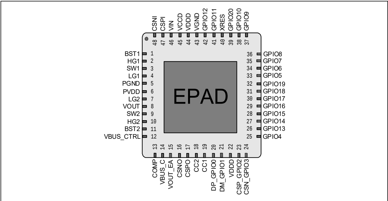
Figure 8 48-QFN pinout
