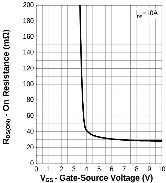
Transfer Characteristics
