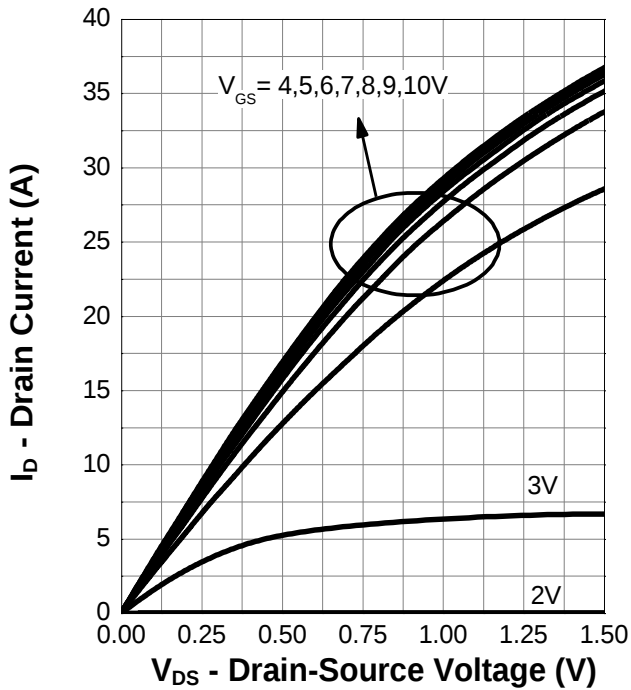
Output Characteristics
