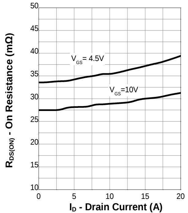
On Resistance
