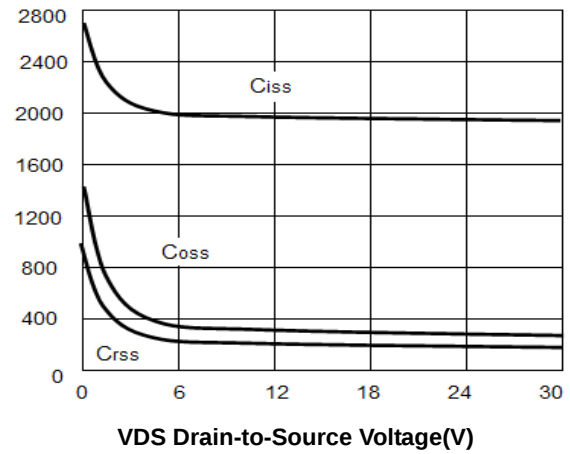
Figure 8. Capacitance
