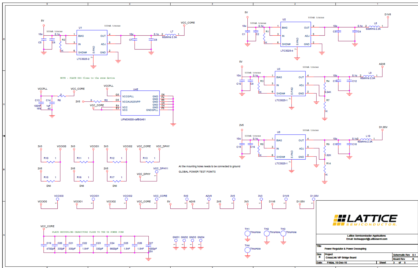
Figure A.2. Power Regulator and Power Decoupling
