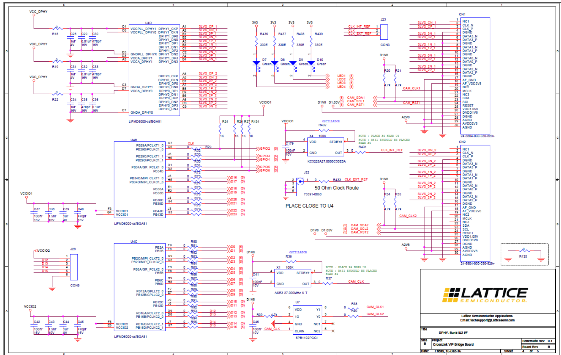
Figure A.3. DPHY, Bank 1 and 2 Interface
