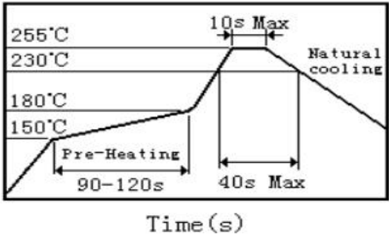
回流焊曲线 Reflow soldering profile
