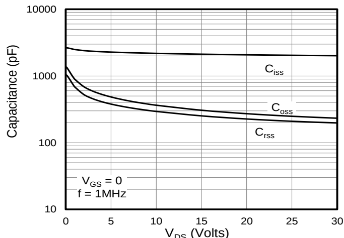
Figure 4: Capacitance Characteristics
