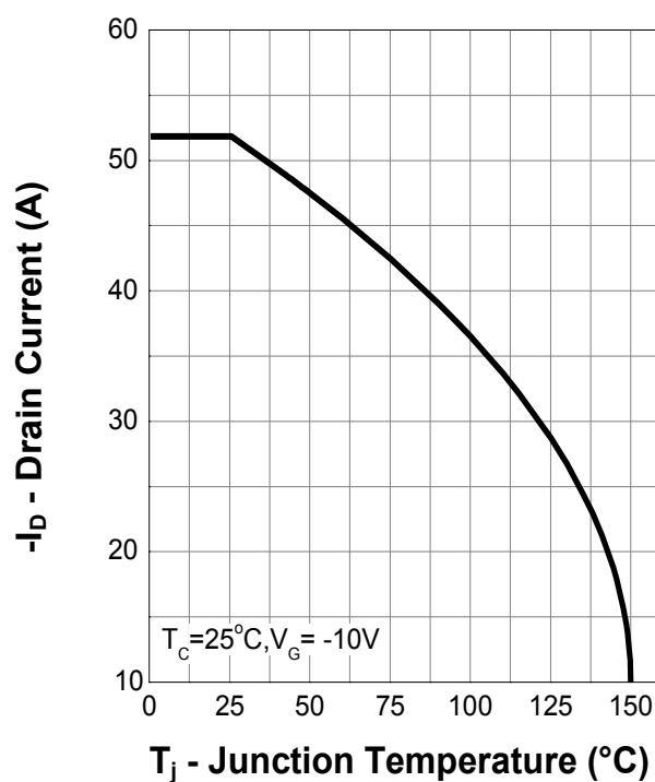
Current Capability
