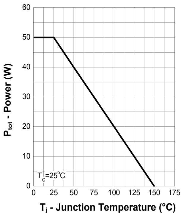
Power Capability
