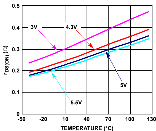
FIGURE 22. ON-RESISTANCE vs TEMPERATURE AT DIFFERENT INPUT VOLTAGES
