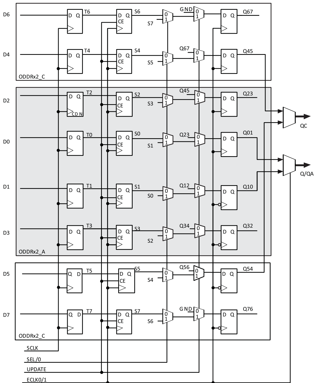
Figure 2.13. Output Gearbox
