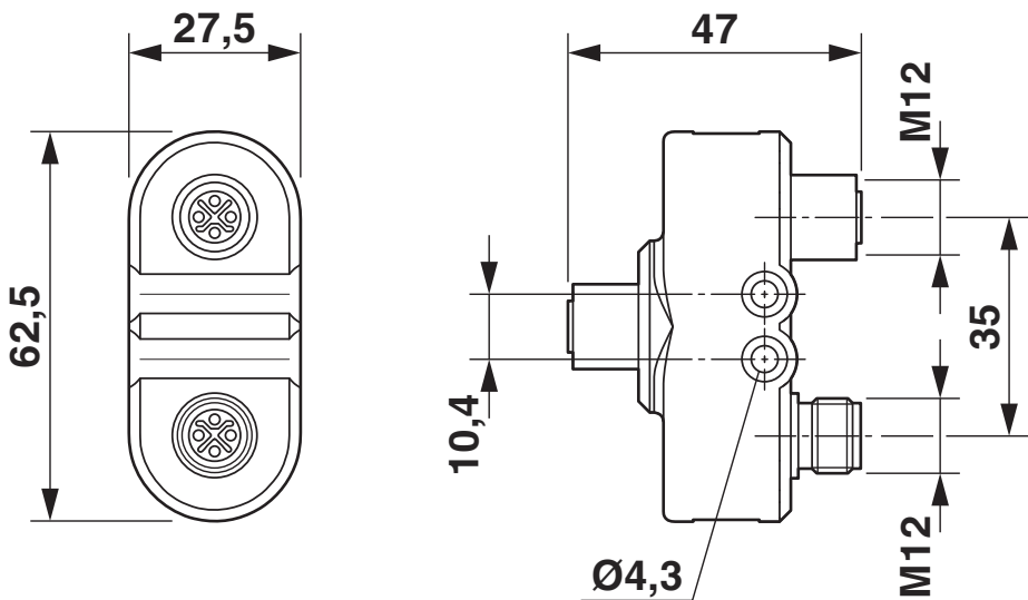
Dimensional drawing
