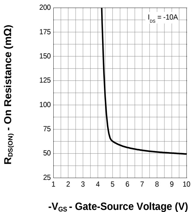
Transfer Characteristics
